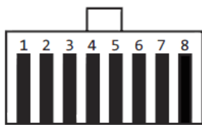
RJ-45/RJ-48/RJ-61 - 8P8C
