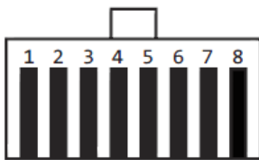
RJ-45/RJ-48/RJ-61 - 8P8C
