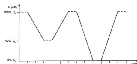
Fig.2: Voltage fluctuation
