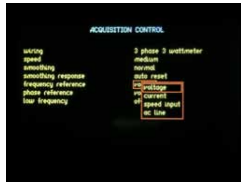
Frequency Reference
